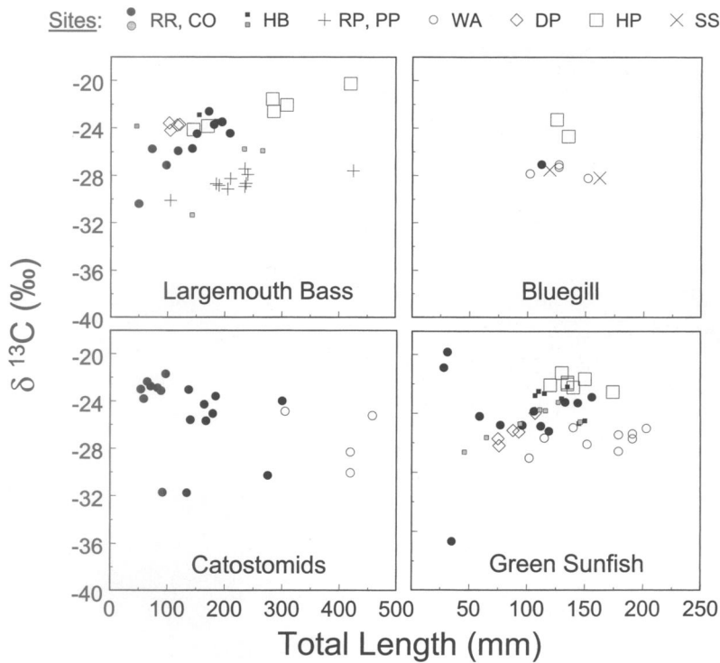
FIG. 2.—Stable carbon ( \delta^{13}\text{C} ) isotope signatures as a function of length of largemouth bass, bluegill, 3 catostomids (bluehead sucker, flannelmouth sucker, white sucker), and green sunfish sampled at backwater (closed symbols; black denotes samples from October, gray denotes samples from April) and pond (open symbols or + and x) sites in the upper Colorado River, 1997 to 1998. See Table 1 for site names and sampling dates.
