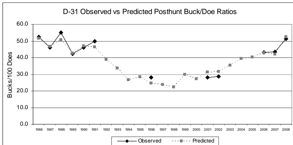
Figure 6. D-31 observed and modeled posthunt sex ratios from 1986 to 2008
